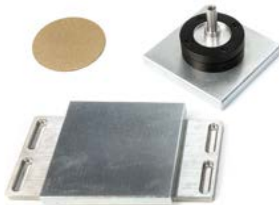
▲ PDV11089 Upper and Lower Compression Plates and self-levelling adapter with circular test piece.
